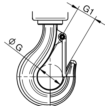
DETAIL Y1
