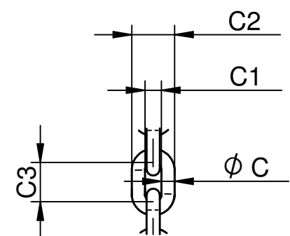
DETAIL Y2
